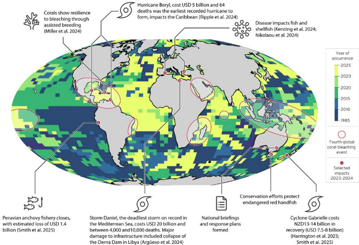
Figure 2. The impacts of the exceptional marine heatwaves in 2023–2024 , which was also the period of occurrence of the warmest sea surface temperature (relative to the seasonal normal) in the satellite record since 1985. Dataset: ESA Climate Change Initiative Sea Surface Temperature v3 (Embury et al. 2024).
