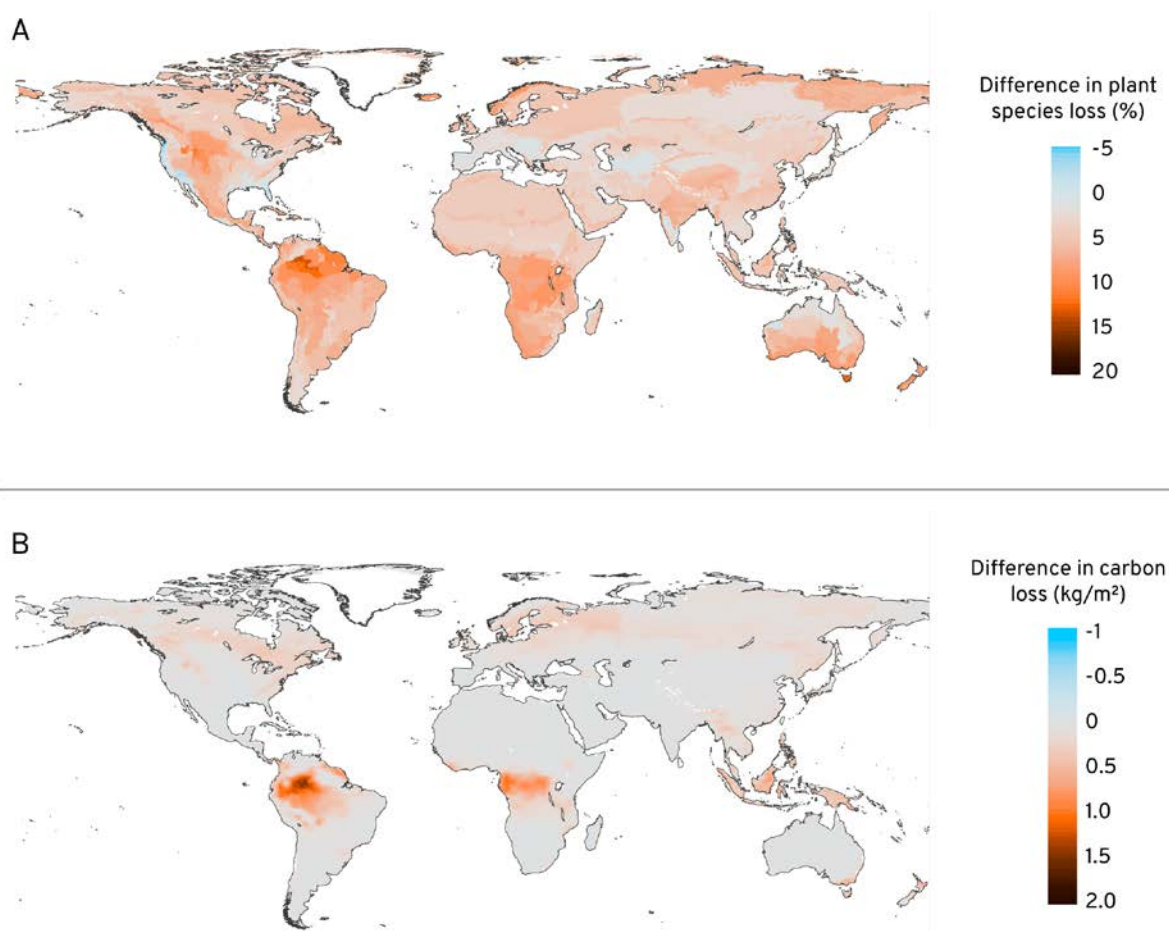
Figure 4. Additional plant diversity loss and resulting carbon loss, under a very high emissions scenario. Long-term loss of vascular plant species richness due to climate change and land use change, projected by 2050 (Panel A), shown as additional percentage of plants lost under a high emissions scenario (RCP8.5) relative to a low emissions scenario (RCP2.6). Reductions in vegetation carbon within the remaining habitat, attributable to plant biodiversity loss (Panel B), shown as additional carbon loss [ \text{kg}/\text{m}^2 ] under high emissions scenario (RCP8.5) relative to a low emissions scenario (RCP2.6) (adapted from Weiskopf et al. 2024).
